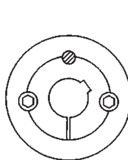
Bush with 2 Grub Screws (Sizes 1008-3030)
