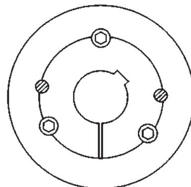
Bush with 3 Grub Screws (Sizes 3535 and above)
