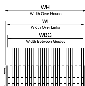
All-Link Assembly
